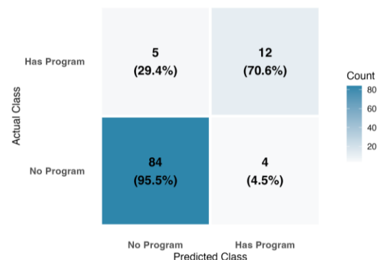
Fig. 8. 10-Fold-Cross-Validation Random Forest Confusion Matrix.
