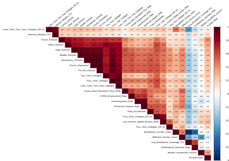
Fig. 9. Predictor + DS/AI College Count Correlation Matrix.
