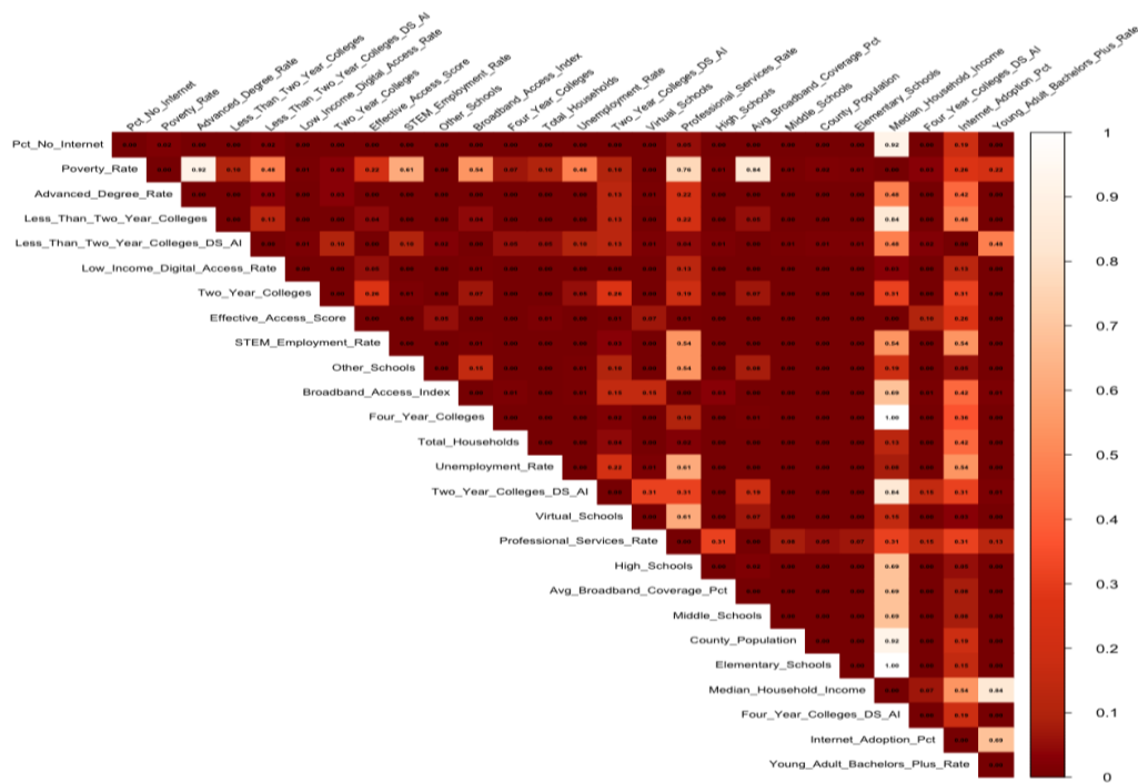
Fig. 10. Predictor + DS/AI College Count P-Value Matrix.
